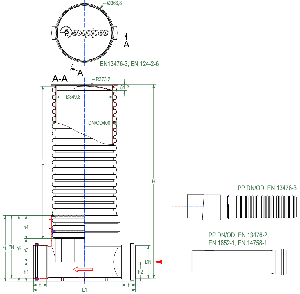
DN400 BASE, TYPE 1B
