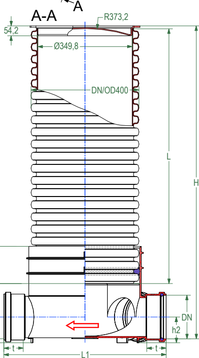
DN400 BASE, TYPE 3BL
