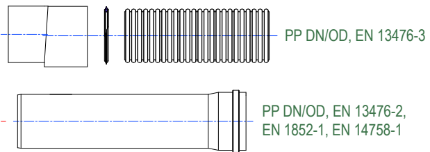
OUT0° / IN135° / IN225° DN110, 160, 200, 250*, 315* mm
