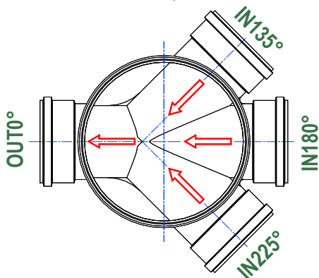
OUT0° / IN135° / IN180° / IN225° DN110, 160, 200, 250*, 315* mm
