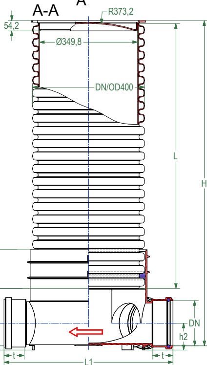
DN400 BASE, TYPE 3BL
