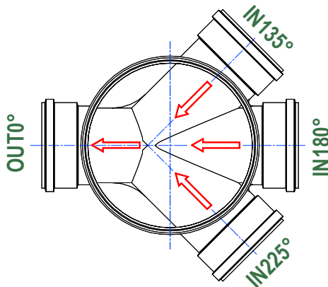
OUT0° / IN135° / IN180° / IN225° DN110, 160, 200, 250*, 315* mm
