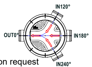
OUT0° / IN180° DN160, 200, 250, 315, 400 mm
