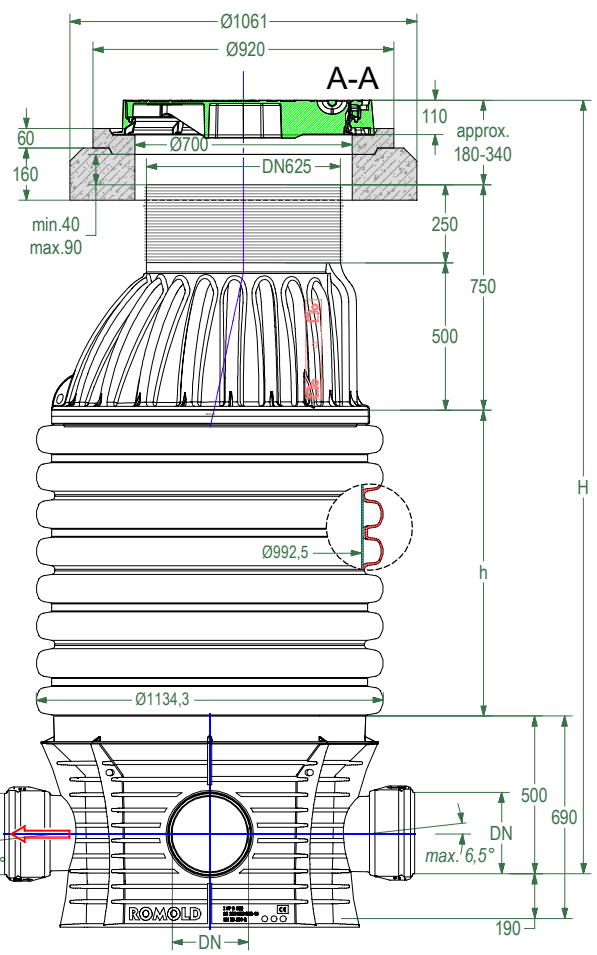
OUT0° / IN90° / IN180° DN160, 200, 250, 315 mm
