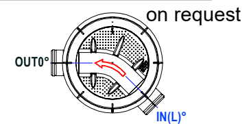
OUT0° / IN(L)° DN160, 200, 250, 315, 400 mm
