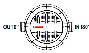
OUT0° / IN180° DN160, 200, 250, 315, 400 mm
