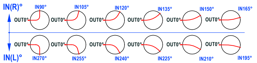
OUT0° / IN(R)° DN160, 200, 250, 315, 400 mm
