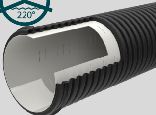
Locally perforated pipe LP(220°±10°)
